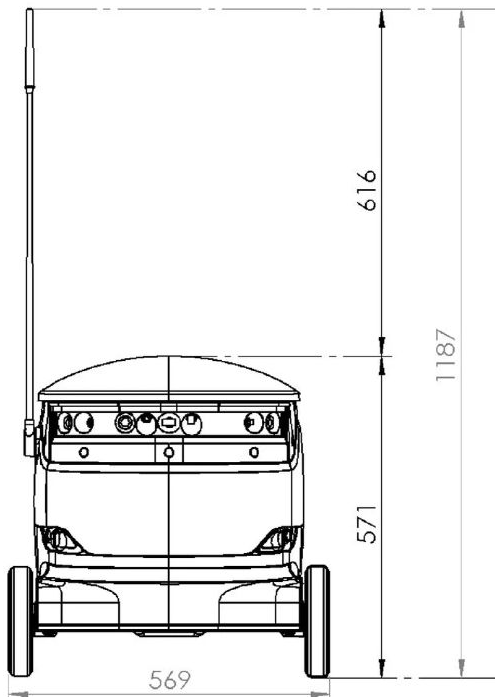
Figure 1: PDD Dimensions from the front
